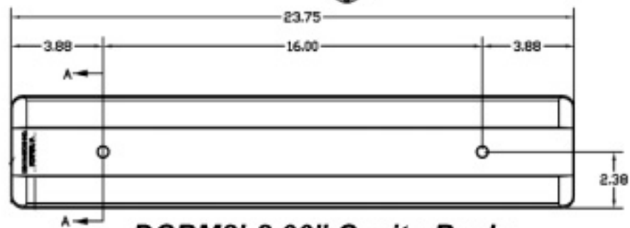
DCBM2'-2.00" Cavity Back
