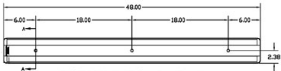
DCBM4'-3.5" Cavity Back
