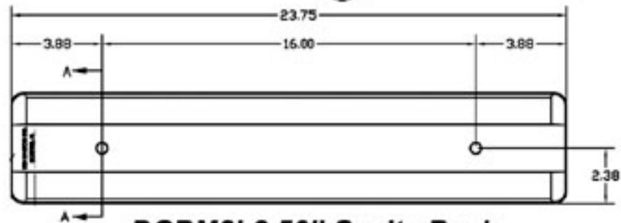
DCBM2'-3.50" Cavity Back
